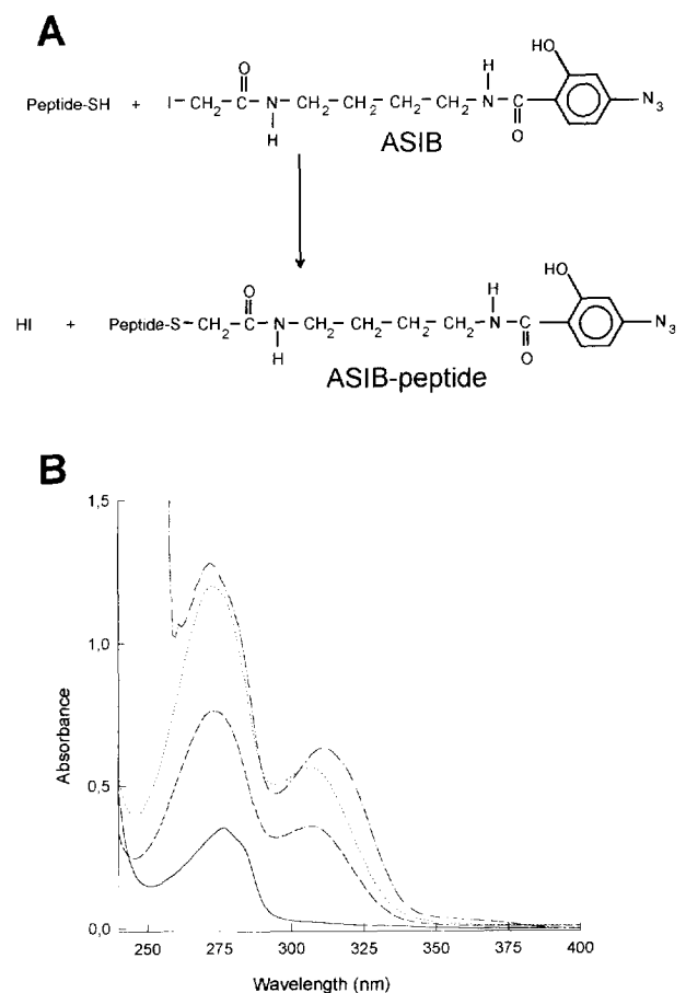
Fig. 1. (A) Scheme of the reaction between 1-( p -azidosalicylamido)-4-(iodoacetamido)butane (ASIB) and a cysteine-containing peptide to yield the corresponding ASIB-peptide. (B) Absorbance spectra of free ASIB (67 \mu M in DMSO) (· · · · ·), ASIB-labeled ShB-21C (38 \mu M in 0.05% acetic acid) (— — —) and ASIB-labeled ShB-L7E-21C (61 \mu M in 0.05% acetic acid) (· · · · ·). The spectrum of unlabeled ShB peptide (250 \mu M in 0.05% acetic acid) (—) is also included to illustrate the contribution of peptide absorbance to the 272 nm maximum.
